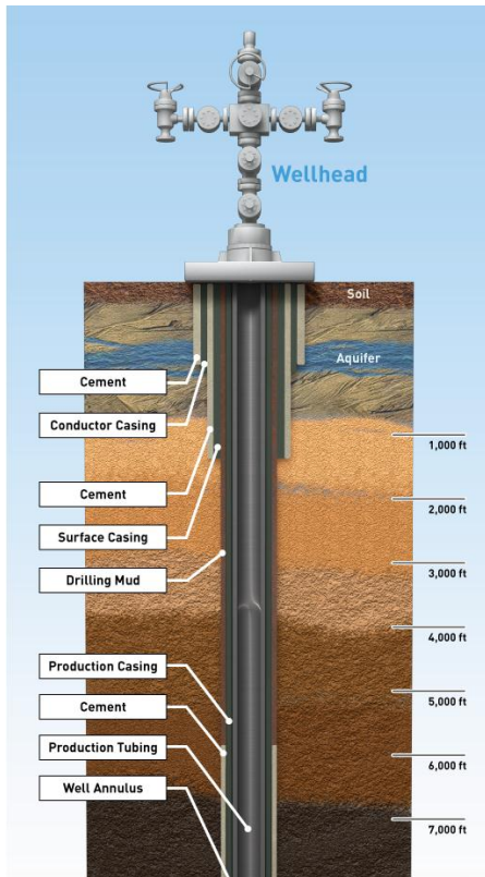
Figure 1: Layers of cement and steel casing of a typical well
